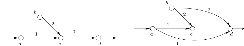
Fig. 10. A Graph with a Zero-Weight Arc and its (Implicit) Transformation.
